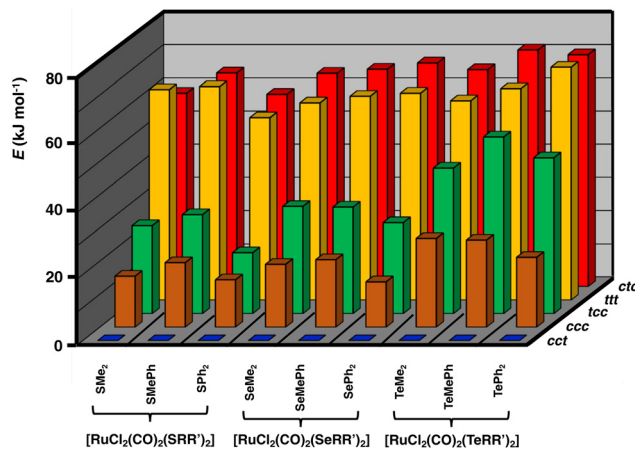
Fig. 2 Relative PBE0/def2-TZVP Gibbs energies (in kJ mol –1 ) of [RuCl 2 (CO) 2 (ERR') 2 ] (E = S, Se, Te; R, R' = Me, Ph). The numerical values of the relative energies are shown in Table S6 in ESI.†
