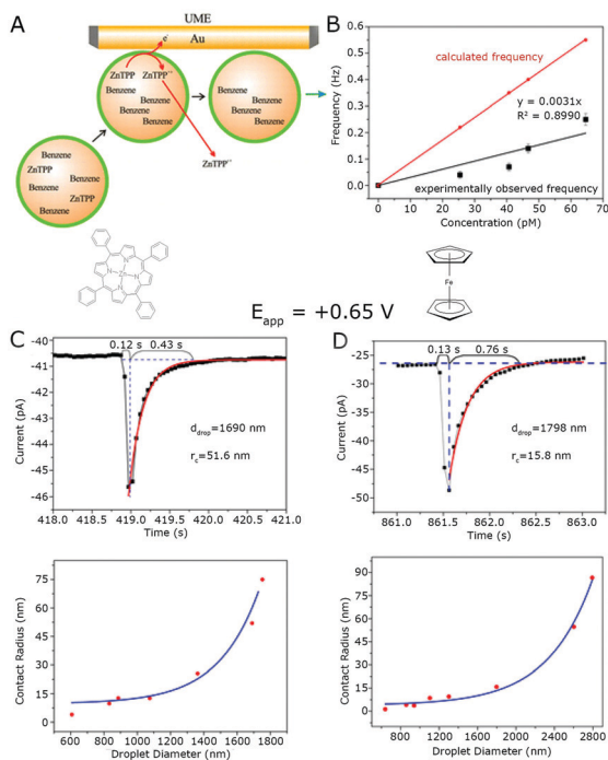
Fig. 29 Single entity impacts of benzene droplets encapsulating different hydrophobic species on Au UME: (A) schematic description of the oxidation of ZnTPP and following escape of ZnTPP •• from the droplet during collision. (B) Comparison of calculated and experimentally observed frequency of collision events at different emulsion concentrations for ZnTPP filled benzene droplets on a 0.65 V vs. Ag/AgCl biased Au UME. (C) Current response of a single ZnTPP containing benzene droplet colliding with the biased Au UME, together with evaluated droplet and droplet/electrode interface-area estimated from eqn (18). Derived droplet/electrode contact radius in dependence of droplet diameter for ZnTPP in benzene nanoemulsions on Au UME at 0.65 V vs. Ag/AgCl. (D) Current response of a single Fc containing benzene droplet colliding with the biased Au UME, together with evaluated droplet and droplet/electrode interface-area estimated from eqn (18). Derived droplet/electrode contact radius in dependence of droplet diameter for Fc in benzene nanoemulsions on Au UME at 0.65 V vs. Ag/AgCl. Reproduced with permission from Y. Li, H. Deng, J. E. Dick and A. J. Bard, Anal. Chem. , 2015, 87 , 11013. 193
