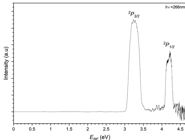
Fig. 8 Photoelectron spectrum of the 169 m/z peak from Fig. 3 assigned to photodetachment to the perturbed ^2P_{3/2} and ^2P_{1/2} states of the \text{I}^{\cdot-}\cdots\text{C}_3\text{H}_6 complex.
