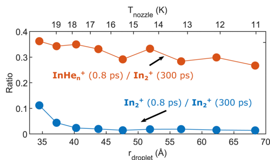
Fig. 8 Droplet size dependence of the \text{InHe}_n^+ and \text{In}_2^+ yields at short pump-probe delays. Both signals are normalized to the \text{In}_2^+ signal at 300 ps delay.
