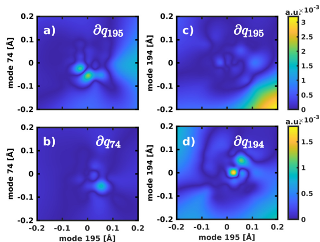
Fig. 6 Visualization of the NACs, projected into the 2D spaces spanned by normal modes 195/74 and 195/194, respectively. The notation \partial q_i refers to the projection of the NACs onto the respective normal mode to yield \langle \Psi_1 | \frac{\partial}{\partial q_i} | \Psi_2 \rangle .
