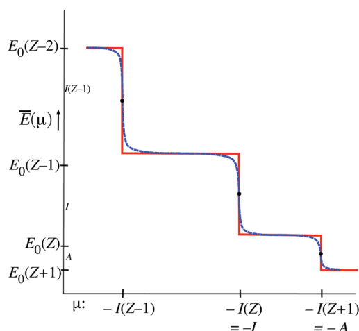
Fig. 4 Step behavior of \bar{E}(\bar{N}) as a function of the parameter \mu for small T (blue dashes) and in the limit T \rightarrow 0 (red lines). For small T the steps are soft. Heavy black dots: values of \bar{E}(\mu) independent of T ; small black dots: values of \bar{E}(\mu) obtained in the limit T \rightarrow 0 only.
