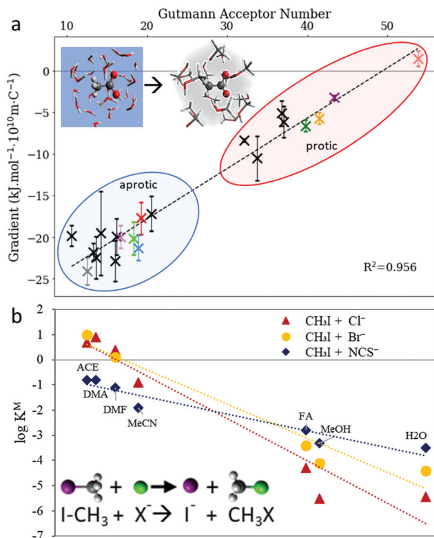
Fig. 15 The Gutmann acceptor number approximates the effect of the solvent on anion trends (a) with the Gibbs free energy of transfer from aqueous to nonaqueous solvents and (b) the S_N2 reaction rate with methyl iodide. Adapted from ref. 128 with permission from the Royal Society of Chemistry, copyright 2021.
