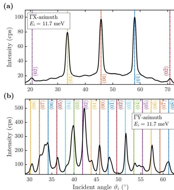
Fig. 2 Diffraction scans along the two high-symmetry directions upon scattering parallel ( \overline{\Gamma}\text{X} (a)) and normal ( \overline{\Gamma}\text{Y} (b)) to the steps, plotted versus incident angle \vartheta_i at a sample temperature of T_s = 113 \text{ K} . The individual diffraction peaks are labelled with the interacting \mathbf{G} -vector.
