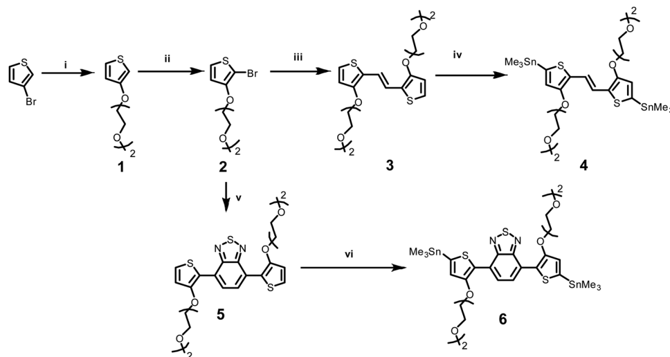
Scheme 1 The synthetic route of bis(trimethylstannyl) glycolated TVT, bis(trimethylstannyl) glycolated TBTT monomers. Reaction conditions: (i) t -BuOK, 2-(2-methoxyethoxy)ethanol, RT, then 100 °C; (ii) NBS, THF/Hexane, 0 °C; (iii) 2-bis(tributylstannyl)ethene, Pd 2 (dba) 3 , P( o -tol) 3 , 100 °C; (iv) n -BuLi, THF, −78 °C, SnClMe 3 , then RT; (v) 4,7-Bis(4,4,5,5-tetramethyl-1,3,2-dioxaborolan-2-yl)2,1,3-benzothiadiazole, Pd 2 (dba) 3 , P( o -tol) 3 , tricaprylylmethylammonium chloride, aq.K 3 PO 4 , toluene; (vi) n -BuLi, THF, −78 °C, SnClMe 3 , then RT.
