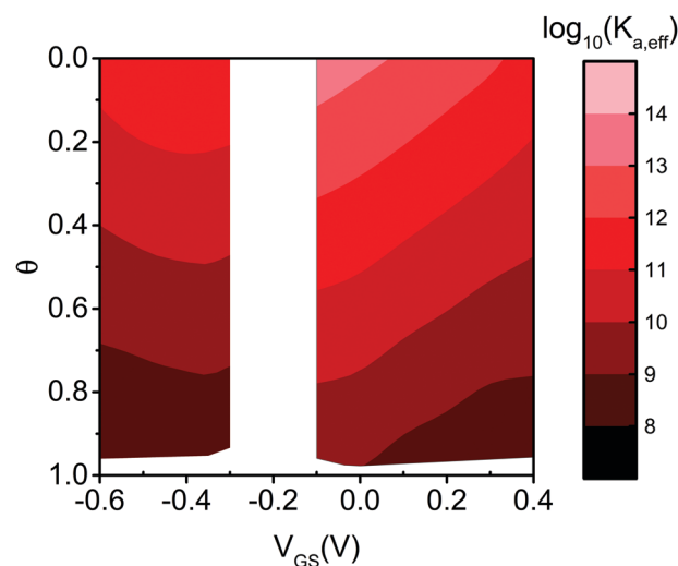
Fig. 5 Contour plot of the effective binding constant as \log_{10}(K_{a,\text{eff}}) as a function of \theta and V_{GS} for EGOFET (left strip) and OECT (right strip).
