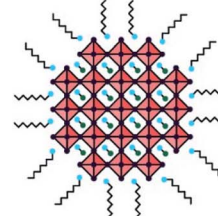
Nanocrystal (0D)
