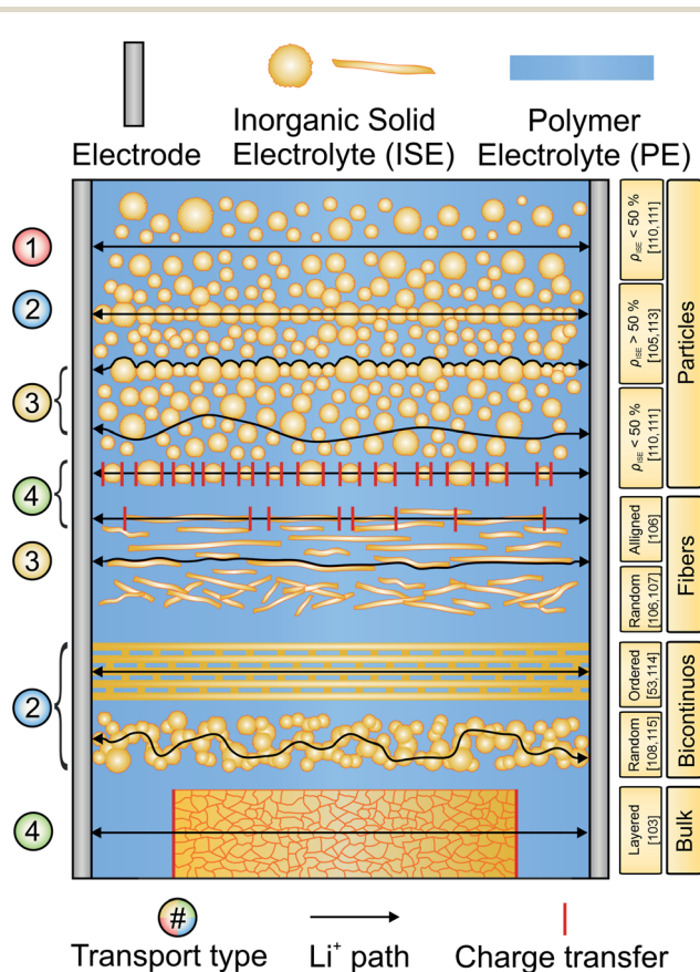
Fig. 7 Schematic representation of the surveyed composite electrolyte architectures. The possible pathways for lithium transport are represented by black lines. In some cases, only one possible pathway is shown for clarity.
