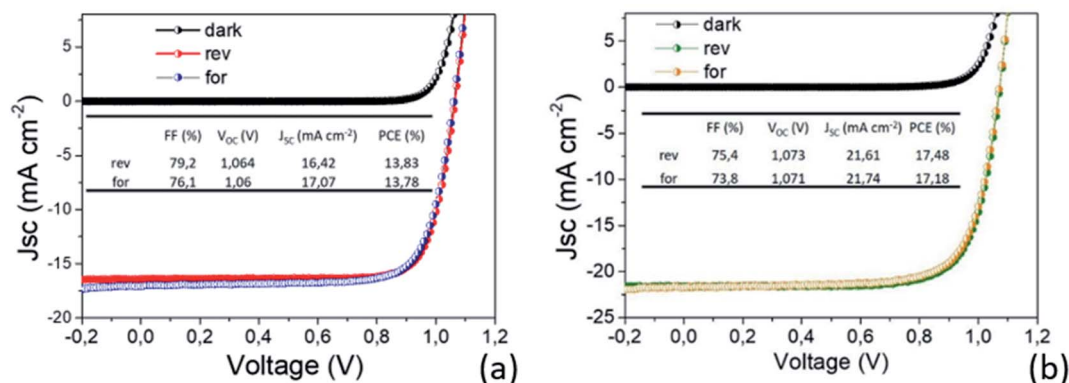
Fig. 9 J – V characterization of the best prepared devices with (a) 80 nm and (b) 150 nm MAPbI 3 active layers. The AVT moves from 32.8% to 20%.
