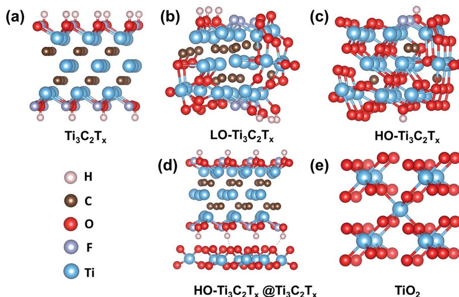
Fig. 5 Predicted crystal structures of \text{Ti}_3\text{C}_2\text{T}_x , \text{LO-Ti}_3\text{C}_2\text{T}_x , \text{HO-Ti}_3\text{C}_2\text{T}_x , \text{HO-Ti}_3\text{C}_2\text{T}_x\text{@Ti}_3\text{C}_2\text{T}_x and \text{TiO}_2 carried out by VASP code based on DFT.
