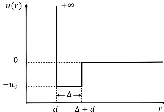
Fig. 1 Pair potential u(r) for sticky hard spheres as a function of inter-particle distance r .
