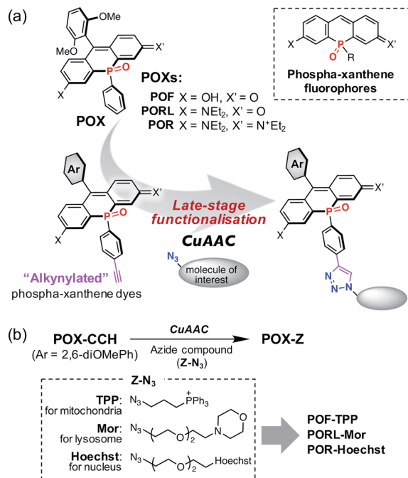
Fig. 1 (a) Functionalisation of phosphaxanthene fluorophores shown in a dashed box. A phenyl ring on the phosphorus atom of the parent POX dyes is modified with an ethynyl group. The alkyne-modified phosphaxanthene dyes thus obtained can be converted into the corresponding triazole compounds via a copper-catalysed azide-alkyne cycloaddition (CuAAC) at the late stage of synthesis. (b) POX-based organelle markers obtained from alkyne-modified-POXs (POX-CCHs) and azide compounds used in this work.
