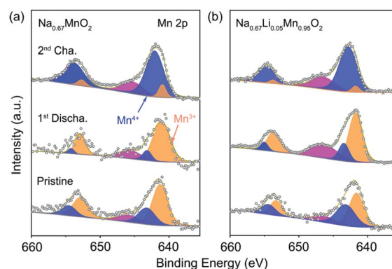
Fig. 3 XPS spectra of Mn 2p collected on the pristine, first discharged and second charged electrode of (a) P'2\text{-Na}_{0.67}\text{MnO}_2 and (b) P'2\text{-Na}_{0.67}\text{Li}_{0.05}\text{Mn}_{0.95}\text{O}_2 .
