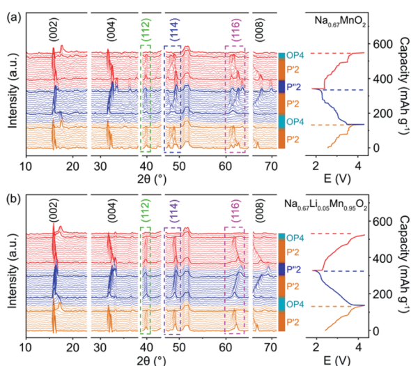
Fig. 2 In situ XRD patterns collected in the first cycle and second charge of (a) P'2\text{-Na}_{0.67}\text{MnO}_2 and (b) P'2\text{-Na}_{0.67}\text{Li}_{0.05}\text{Mn}_{0.95}\text{O}_2 .
