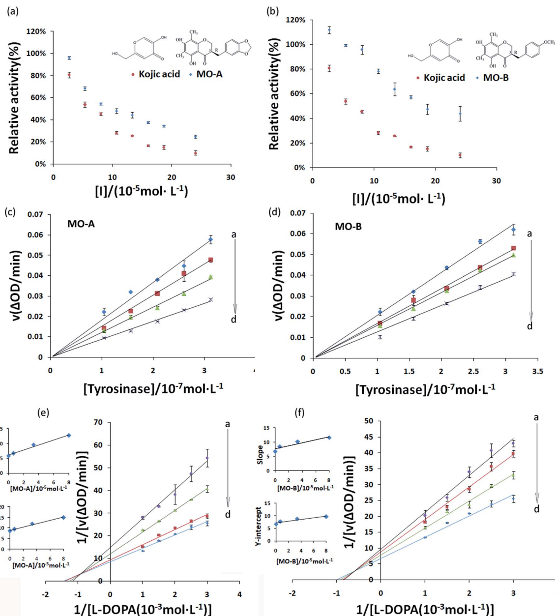
Fig. 1 (a, b) Inhibitory effects of MO-A(A), MO-B(B) on Tyr; c(\text{Tyr}) = 2.08 \times 10^{-7} \text{ mol L}^{-1} , and c(\text{L-dopa}) = 5.0 \times 10^{-4} \text{ mol L}^{-1} . (c, d) Types of Tyr inhibition by MO-A (c) and MO-B (d); c(\text{L-dopa}) = 5.0 \times 10^{-4} \text{ mol L}^{-1} , and c(\text{MO-A/MO-B}) = 0, 0.67, 3.33, \text{ and } 8.0 \times 10^{-5} \text{ mol L}^{-1} for curves a \rightarrow d, respectively. (e, f) Lineweaver-Burk plots for MO-A (e) and MO-B (f). c(\text{Tyr}) = 2.08 \times 10^{-7} \text{ mol L}^{-1} ; concentrations of MO-A, B corresponding to curves a \rightarrow d were 0, 0.67, 3.33 \text{ and } 8.0 \times 10^{-5} \text{ mol L}^{-1} . The secondary replots of slope versus [Tyr] and Y-intercept versus [Tyr] were in the inset.
