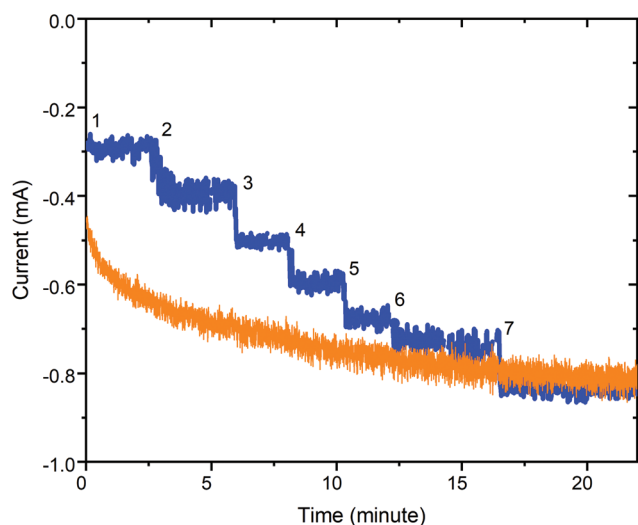
Fig. 11 Plot of current response versus time at E = -1.6 V vs. \text{Ag}/\text{AgNO}_3 ( 0.01 M) for a 0.33 M acetonitrile solution of 1 when the acetic acid is either (blue) added in 7 portions reaching 80 mM in \text{H}^+ after the 7^{\text{th}} addition or (orange) it is 80 mM from the start. Conditions: Glassy carbon working electrode ( d = 3 mm, A = 0.071 cm ^2 ), 20 °C, and Pt counter electrode. Also see Table S3.†
