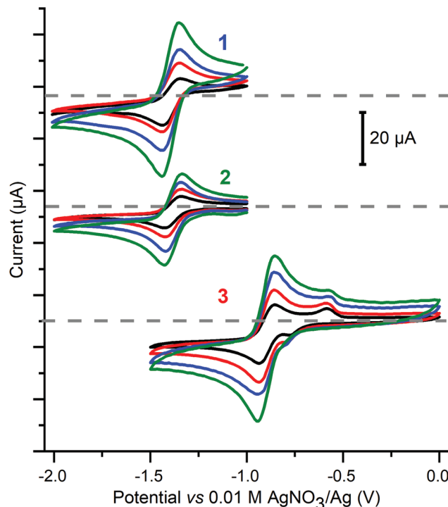
Fig. 7 Cyclic voltammetry of the reversible redox processes seen at negative potentials for 1 \text{ mM} MeCN solutions of 1 (top, E_{1/2} = -1.39 \text{ V} , \Delta E = 0.09 \text{ V} , D = 7.7 \times 10^{-6} \text{ cm}^2 \text{ s}^{-1} ), 2 (middle, E_{1/2} = -1.39 \text{ V} , \Delta E = 0.09 \text{ V} , D = 3.4 \times 10^{-6} \text{ cm}^2 \text{ s}^{-1} ), and 3 (bottom, E_{1/2} = -0.89 \text{ V} , \Delta E = 0.09 \text{ V} , D = 5.4 \times 10^{-6} \text{ cm}^2 \text{ s}^{-1} ). Conditions: 0.1 \text{ M} (\text{Bu}_4\text{N})\text{PF}_6 , glassy carbon working electrode ( d = 3 \text{ mm} , A = 0.071 \text{ cm}^2 ), 293 \text{ K} , vs. 0.01 \text{ M} \text{AgNO}_3/\text{Ag} . In this system E_{1/2}(\text{Fc}^+/\text{Fc}) = 0.09 \pm 0.01 \text{ V} , with \Delta E = 0.09 \text{ V} , and this was unchanged even after 6 \text{ h} of electrolysis (Fig. S31†). Scan direction: for 1 and 2 -1.0 \rightarrow -2.0 \rightarrow -1.0 \text{ V} , for 3 0.0 \rightarrow -1.5 \rightarrow 0.0 \text{ V} ; scan rate: 50 (black), 100 (red), 200 (blue) and 400 (green) \text{mV s}^{-1} ; grey dashed lines correspond to zero current for each set of CVs.
