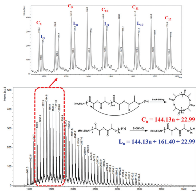
Fig. 4 MALDI-TOF mass spectrum (major population: Na + ) of the PLA sample ( M_{n, GPC} = 2900 \text{ g mol}^{-1} , M_w/M_n = 1.88 ) prepared with catalyst 1 ( C(\text{cyclic}) = 144.13n + 22.99 , L(\text{linear}) = 144.13n + 161.40 + 22.99 , where n is the degree of polymerization, M_{LA} = 144.13 \text{ g mol}^{-1} , M_{NH(SiMe_3)_2} = 161.40 \text{ g mol}^{-1} , M_{Na} = 22.99 \text{ g mol}^{-1} ).
