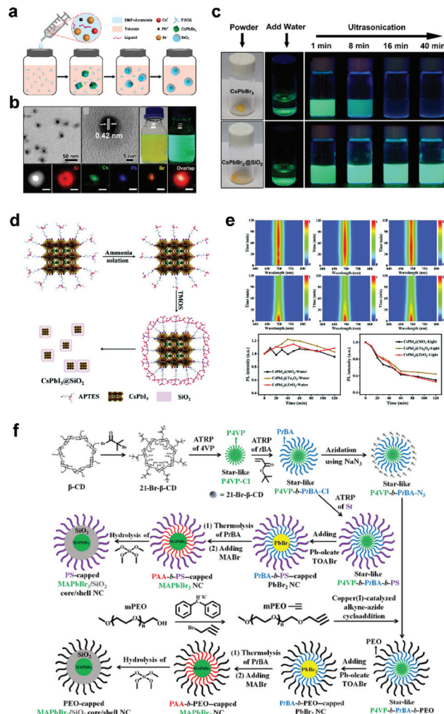
Fig. 3 (a) Formation process of \text{CsPbBr}_3/\text{SiO}_2 core/shell NCs. (b) TEM and EDS mapping images of \text{CsPbBr}_3/\text{SiO}_2 core/shell NCs. (c) High stability of \text{CsPbBr}_3/\text{SiO}_2 core/shell NCs against water treatment. Reproduced with permission from ref. 26. Copyright 2018 American Chemistry Society. (d) Synthetic strategy for \text{CsPbI}_3/\text{SiO}_2 core/shell NCs using APTES as a linking ligand. (e) High stability of \text{CsPbI}_3/\text{SiO}_2 core/shell NCs against water treatment. Reproduced with permission from ref. 28. Copyright 2021 Royal Society of Chemistry. (f) Stepwise representation of the synthetic route to PS-capped \text{MAPbBr}_3/\text{SiO}_2 core/shell NCs and PEO-capped \text{MAPbBr}_3/\text{SiO}_2 core/shell NCs by exploiting the star-like \text{P4VP-}b\text{-PtBA-}b\text{-PS} and \text{P4VP-}b\text{-PtBA-}b\text{-PEO} as nanoreactors, respectively. CD, cyclodextrin; BMP, 2-bromo-2-methylpropionate; and TOABr, tetraoctylammonium bromide. Reproduced with permission from ref. 49. Copyright 2019 Creative.
