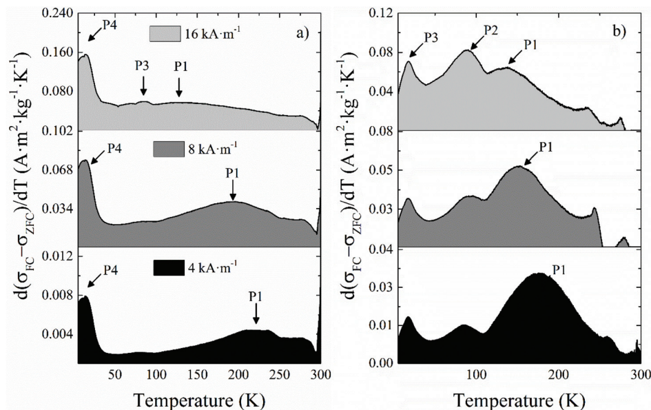
Fig. 5 Differential ZFC magnetization curves with respect to the temperature for samples (a) NO18 and (b) NS18 obtained at external fields of 4, 8 and 16 kA \cdot m^{-1} .
