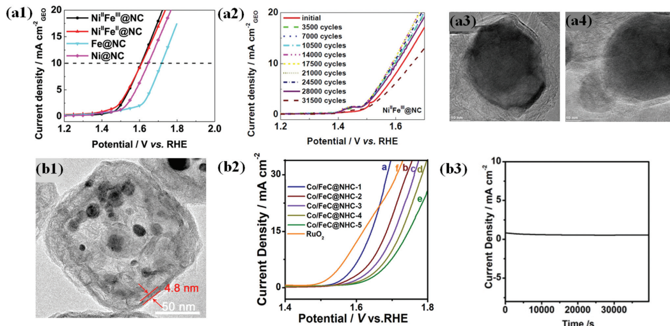
Fig. 9 (a1) LSV curves (10 mV s -1 @900 rpm) of Ni II Fe III @NC, Ni II Fe II @NC, Fe 4 [Fe II (CN) 6 ] 3 derived Fe@NC and Ni II [Ni II (CN) 4 ] derived Ni@NC catalysts in oxygen-saturated 0.1 M KOH solutions. (a2) LSV curves of Ni II Fe III @NC after a certain number of ADT cycles between 1.2 and 1.9 V at 500 mV s -1 . TEM images of (a3) Ni II Fe III @NC and (a4) Ni II Fe III @NC catalysts after ADT, reproduced with permission from ref. 63, Elsevier copyright 2017. (b1) TEM images of (A) Co/FeC@NHC-1 (b2) OER polarization curves of Co/FeC@NHC-1, Co/FeC@NHC-2, Co/FeC@NHC-3, Co/FeC@NHC-4, Co/FeC@NHC-5, and RuO 2 in 1 M KOH. (b3) Potentiostatic response (current density versus time) under a constant potential of 1.54 V vs. RHE, reproduced with permission from ref. 151, Elsevier copyright 2020.
