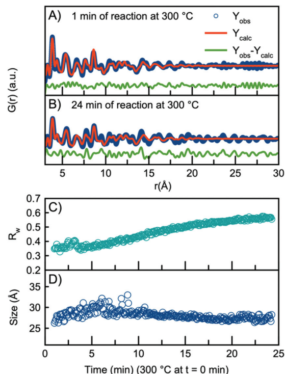
Fig. 3 PDF fit using the \text{H-Nb}_2\text{O}_5 structure to the data collected (A) after 1 min of reaction and (B) 24 min of reaction. (C) R_w values obtained from sequential refinement with \text{H-Nb}_2\text{O}_5 plotted as a function of time. (D) The refined crystallite size plotted as a function of time.
