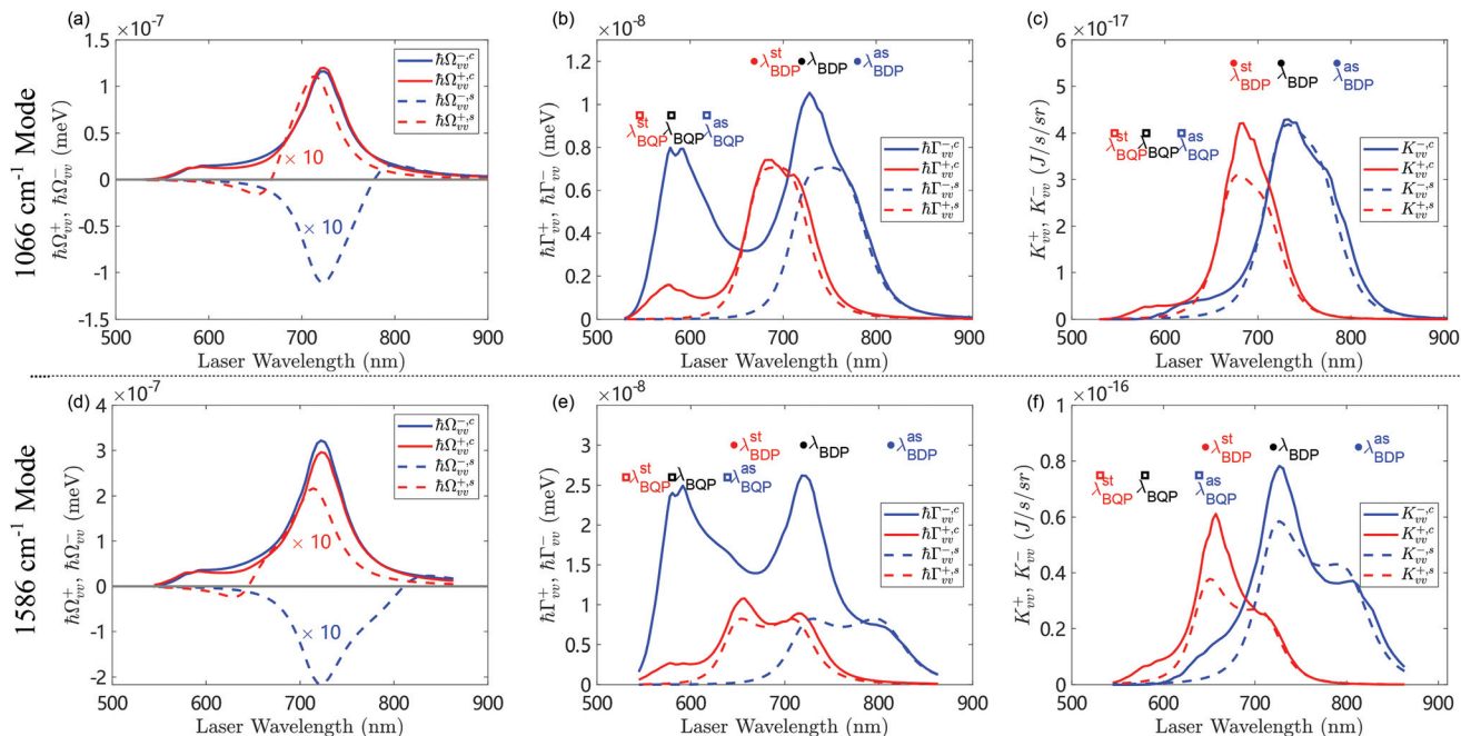
Fig. 4 Dependence of (a and d) the vibrational frequency shift parameters \Omega_{\text{W}}^{\pm, c} , \Omega_{\text{W}}^{\pm, s} , (b and e) the vibrational pumping \Gamma_{\text{W}}^{+, c} , \Gamma_{\text{W}}^{+, s} and damping \Gamma_{\text{W}}^{-, c} , \Gamma_{\text{W}}^{-, s} rates, and (c and f) the propagation factors K_{\text{W}}^{\pm, c} , K_{\text{W}}^{\pm, s} , on the wavelength of the illuminating laser of intensity I_{\text{las}} = 1 \mu\text{W} \mu\text{m}^{-2} and Raman-active vibrational mode of wave-number (a–c) 1066 \text{cm}^{-1} and (d–f) 1586 \text{cm}^{-1} . The solid lines are computed with the continuum-field model (labeled by “c”) while the dashed lines are calculated with the single-mode model (labeled by “s”). In (b and c), the dots from right to left mark the laser wavelengths where the anti-Stokes emission ( \lambda_{\text{BDP}}^{\text{st}} = 780 \text{ nm} ), the excitation ( \lambda_{\text{BDP}} = 720 \text{ nm} ), and the Stokes emission ( \lambda_{\text{BDP}}^{\text{st}} = 669 \text{ nm} ) are maximized due to the BDP mode. The squares mark the same information ( \lambda_{\text{BQP}}^{\text{st}} = 618 \text{ nm} , \lambda_{\text{BQP}} = 580 \text{ nm} , \lambda_{\text{BQP}}^{\text{st}} = 546 \text{ nm} ) for the BQP mode. In (e and f), the dots and squares mark the same information as in (b and c) for the high-energy vibrational mode with values of \lambda_{\text{BDP}}^{\text{st}} = 813 \text{ nm} , \lambda_{\text{BDP}} = 720 \text{ nm} , and \lambda_{\text{BDP}}^{\text{st}} = 646 \text{ nm} for the BDP mode, and \lambda_{\text{BQP}}^{\text{st}} = 639 \text{ nm} , \lambda_{\text{BQP}} = 580 \text{ nm} , and \lambda_{\text{BQP}}^{\text{st}} = 531 \text{ nm} for the BQP mode. The difference between the wavelengths marked in (b and c) and (e and f) are due to the difference in the vibrational energy, which affects the Stokes and anti-Stokes frequencies. The results for the 1269 \text{cm}^{-1} mode are shown in Fig. S4 of the ESI.† Other parameters are specified in the text.
