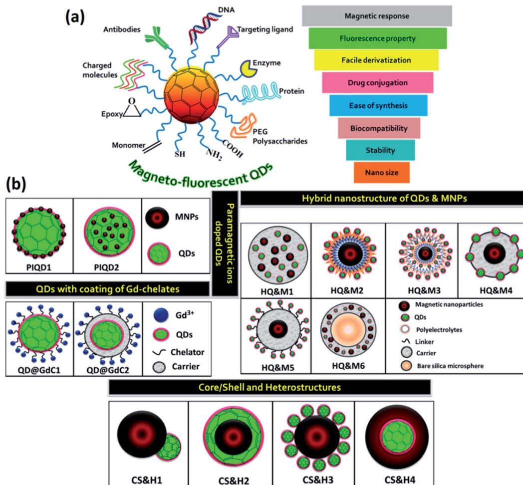
Fig. 1 (a) Overview of the unique properties of MFQDs rendering them excellent candidacy for biomedicine, magnetic imaging, and cancer therapeutics. (b) Schematic representation of different types of MFQDs.
