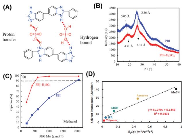
Fig. 5 (A) Reaction mechanism of PBI interaction with acids such as \text{H}_2\text{SO}_4 using H-bonding and proton transfer mechanisms, (B) changes in d -spacing for PBI and \text{H}_2\text{SO}_4 cross-linked PBI hollow fibers (HF) using XRD, and (C) MWCO measurement for PBI and \text{H}_2\text{SO}_4 cross-linked PBI using PEG isomers. 32 Copyright 2019, Elsevier. (D) Relationship between solvent permeance against Hansen solubility parameter ( \delta_p ), viscosity ( \eta ), and molar volume ( V ) of solvent. 34 Copyright 2018, Elsevier.
