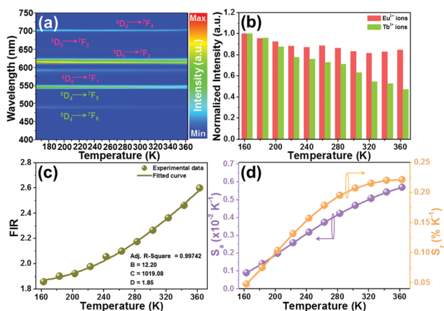
Fig. 5 (a) Thermal evolution emission spectra of YMO: Tb^{3+}/0.06Eu^{3+} NTE microparticles excited at 297 nm. (b) Normalized emission intensities of the Eu^{3+} and Tb^{3+} ions as a function of temperature. (c) Dependence of FIR value on temperature. (d) Temperature-dependent S_a and S_r values.
