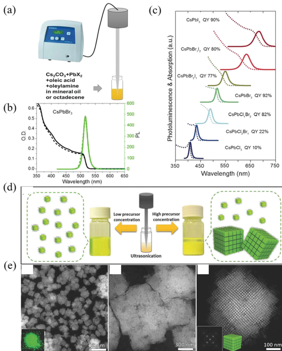
Fig. 4 (a) Synthesis of CsPbX 3 NCs through single-step tip sonication. (b) Absorption (black line) and PL spectra (green line) of fresh (solid line) and 4 months aged (dashed line) CsPbBr 3 colloidal solution. It can be seen that the fresh and aged samples show similar absorption onsets and PL peak positions, while only a small decrease in the PL intensity is seen in the aged sample, indicating the good long-term stability of the colloidal NCs. (c) The corresponding UV/Vis and PL spectra and PLQYs of the samples (Reproduced from ref. 41 with permission from 2016 Wiley-VCH). (d) Schematic illustration of the synthesis of the CsPbBr 3 perovskite NCs by single-step tip sonication of the precursor salts in octadecene. The reaction yields well-dispersed individual NCs at low precursor concentration (left side), while it results in the formation of self-assembled SCs for high precursor concentrations (right side). (e) HAADF-STEM images of the colloidal SCs (Reproduced from ref. 42 with permission from 2018 Wiley-VCH).
