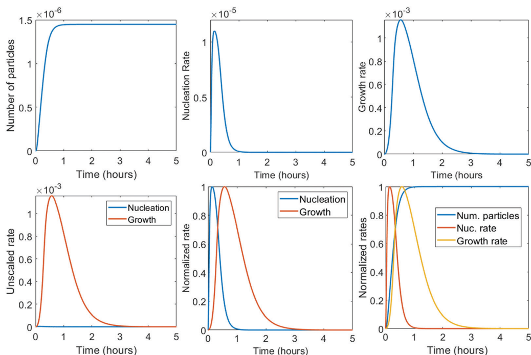
Fig. 27 Numerically calculated number of particles (M), nucleation rate (M h -1 ), and growth rate (M h -1 ) for the 3-step mechanism with the experimentally established nucleation mechanism (“alternative termolecular nucleation” 26,61,62 ) used to construct the mechanism-enabled population balance model. Both unscaled (top) and scaled (bottom) versions of the results from the ME-PBM are shown. The number of particles increases monotonically demonstrating the continuous nucleation of particles. The nucleation rate spikes, and appears “burst-like”, but actually involves kinetically continuous nucleation. The burst feature is actually due to burst-like autocatalytic growth, as shown in the bottom-left figure. The spike periods of nucleation and growth where the two rates are both relatively very high overlap for approximately one fifth of the measured time. Reproduced with permission from ref. 62. Copyright 2020 American Chemical Society.
