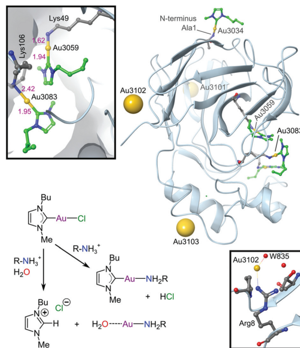
Fig. 15 X-ray structure (1.70 Å resolution) of the Au(I)-NHC adduct with thaumatin (PDB 5JYX). The three Au(I) ions bound to surface residues (Arg8, Lys97, Arg175) are indicated by large spheres. These Au(I) ions have water weakly coordinated trans to the protein N-donor ligand and the NHC has dissociated (presumably as the protonated imidazolium ion). Coordination of Au(I) to Arg8 and water 835 is indicated (lower inset) to illustrate a surface-bound NHC-free Au(I) ion. Three other amino groups (Ala1, Lys49, and Lys106) are coordinated to Au(I)-NHC moieties (green carbon atoms). The upper inset displays the coordination environments for the Au(I)-NHC moieties bound to Lys49 and Lys106. The reaction scheme summarizes the most likely coordination chemistry for the system.
