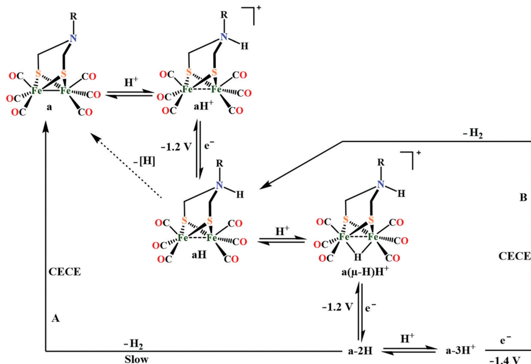
Scheme 26 Proposed mechanisms of proton reduction catalysed by [\text{Fe}_2(\text{CO})_6(\mu\text{-SCH}_2\text{NH}(\text{R})\text{CH}_2\text{S})] complexes (R = \text{CH}_2\text{CH}_2\text{OMe} , Fig. 28a) in MeCN. 426
