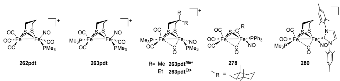
Fig. 85 Exemplary nitrosyl substituted complexes. Note: in the crystalline state 263\text{pdt} shows different degrees of rotation.
