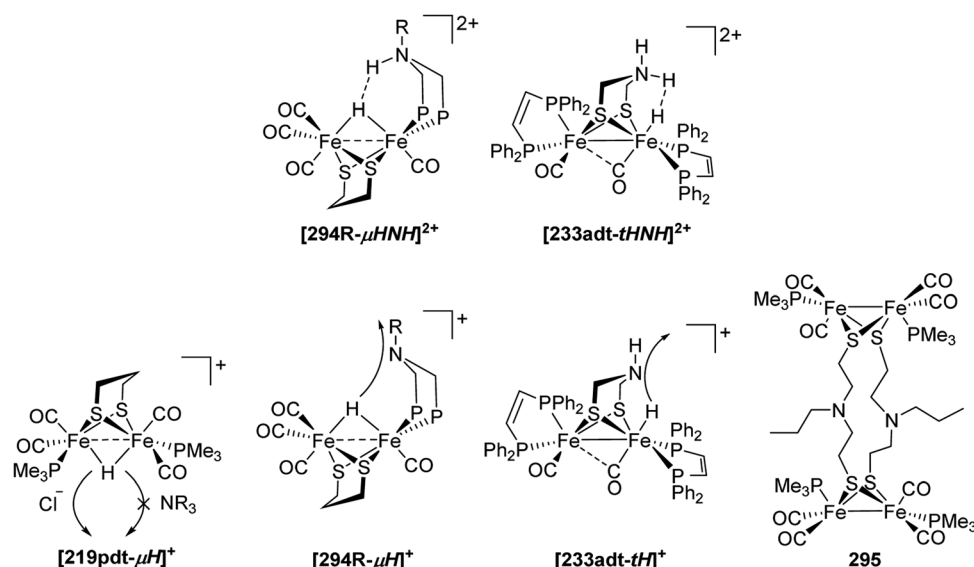
Fig. 93 Top: H-H interaction in double-protonated complexes. Bottom: Deprotonation of hydride complexes and structure of complex 295 (Note: \text{P} = \text{PPh}_2 in 294R ).
