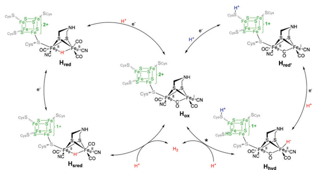
Fig. 20 Shortened catalytic cycle A from Fig. 3.11 and secondary cycle B, which is based on bridging hydrides. Red protons: catalytic PTP, blue proton: accessory PTP. H_{oxH} might be involved in this conversion.
