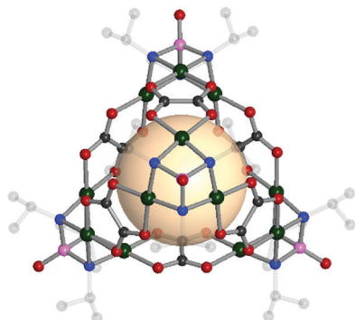
Fig. 10 Structural illustration of [(\text{Pd}_3\text{I}(\text{N}^i\text{Pr})_3\text{PO})_4(\text{A19})_6]^{60}
