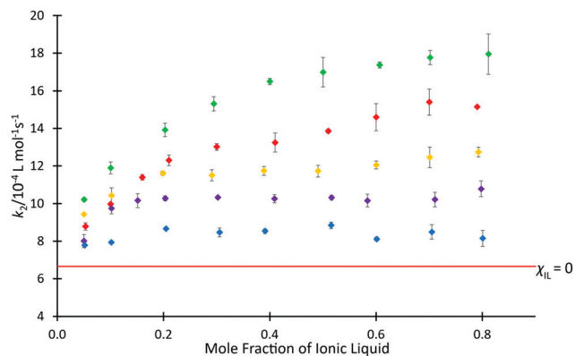
Fig. 3 The bimolecular rate coefficient ( k_2 ) for the reaction of benzyl bromide 1 and pyridine 2 at 22.2 °C in mixtures containing different proportions of either [C_2C_1\text{im}][\text{N}(\text{SO}_2\text{CF}_3)_2] 4a ( \blacklozenge ), [C_4C_1\text{im}][\text{N}(\text{SO}_2\text{CF}_3)_2] 4b ( \blacklozenge ), 37 [C_6C_1\text{im}][\text{N}(\text{SO}_2\text{CF}_3)_2] 4c ( \blacklozenge ), [C_8C_1\text{im}][\text{N}(\text{SO}_2\text{CF}_3)_2] 4d ( \blacklozenge ), or [C_{12}C_1\text{im}][\text{N}(\text{SO}_2\text{CF}_3)_2] 4f ( \blacklozenge ) in acetonitrile, and in acetonitrile ( \rightarrow ). Uncertainties are reported as the standard deviation of at least triplicate results. Some uncertainties fall within the size of the markers used.
