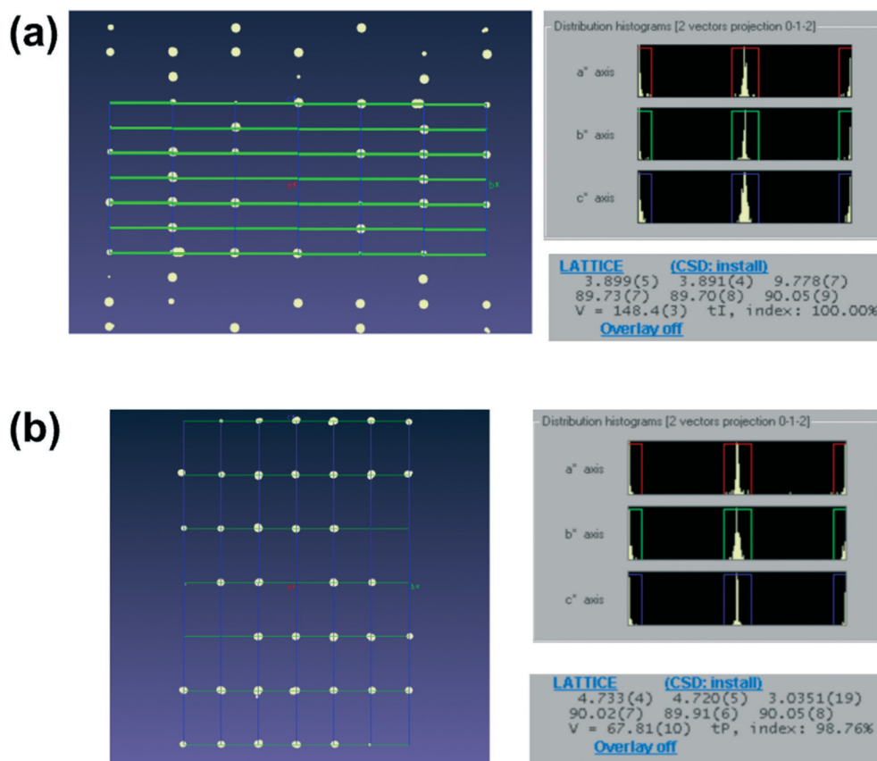
Fig. 4 Detection of polymorphism in TiO 2 by comparing the unit cells it was confirmed that anatase and rutile microcrystals can be distinguished by 3D ED/microED. Distribution of reciprocal lattice points ( a axis projection) and unit cell for (a) anatase and (b) rutile. In both (a) and (b), the diffraction spots are at the intersections of the unit cells represented by the grid points in the figures (left figures), therefore the indexings were probably correct. In addition, the unit cell of the two crystals was determined with very high index rates (100.0% and 98.76% respectively).
