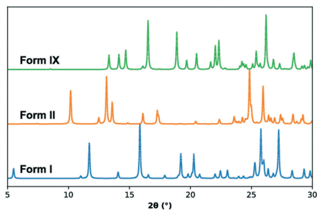
Fig. 3 Simulated PXRD patterns for form I (KAXXA101, blue), form II (KAXXAI, orange) and form IX (this study, green) TFA.
