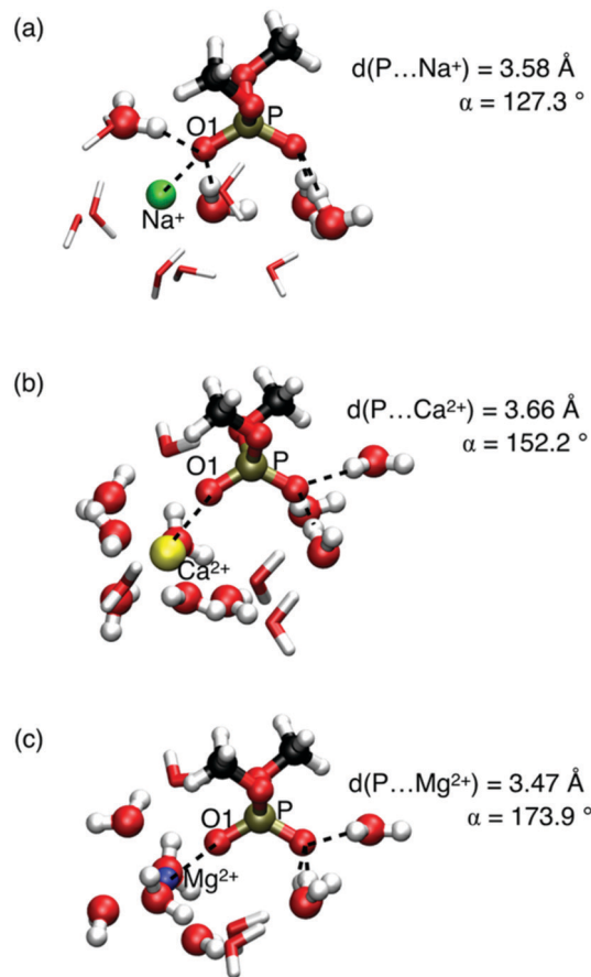
Fig. 8 DMP (\text{H}_2\text{O})_N\text{M}^{x+} cluster geometries ( \text{M}^{x+} = \text{Na}^+, \text{Mg}^{2+}, N = 11 ; \text{M}^{x+} = \text{Ca}^{2+}, N = 13 ). Water molecules of the first hydration shell around the ions and hydrogen bonded water molecules with DMP in ball-and-stick representation; the O1 atom of the (\text{PO}_2)^- group replaces one of the water oxygen atoms in the octahedral solvation geometry around the \text{Mg}^{2+} ion. Vibrational frequencies \nu_{\text{AS}}(\text{PO}_2)^- of structures shown in a, b and c are 1208, 1226, and 1248 \text{cm}^{-1} , respectively. Adapted with permission from ref. 65. Copyright 2019 American Chemical Society.
