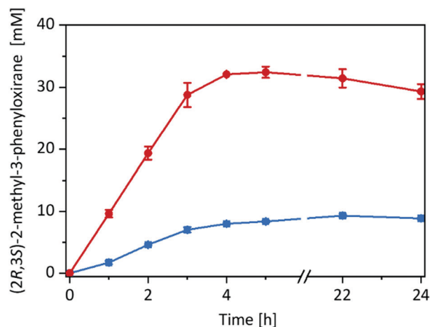
Fig. 2 Product formation over time for the epoxidation of cis - \beta -methylstyrene in different reaction systems: imm- rAaeUPO in neat substrate (180 mg immobilisate in 570 \mu L cis - \beta -methylstyrene) (red circles), and free rAaeUPO in a two-liquid phase system (180 \mu L TRIS-HCl buffer (20 mM, pH 7): 570 \mu L cis - \beta -methylstyrene) (blue squares). General reaction conditions: [ rAaeUPO ] = 0.5 \mu M, t BuOOH feeding rate = 10 mM h -1 , room temperature, shaking at 99 rpm with 60° angle in an overhead rotator. Data represents the average of duplicates.
