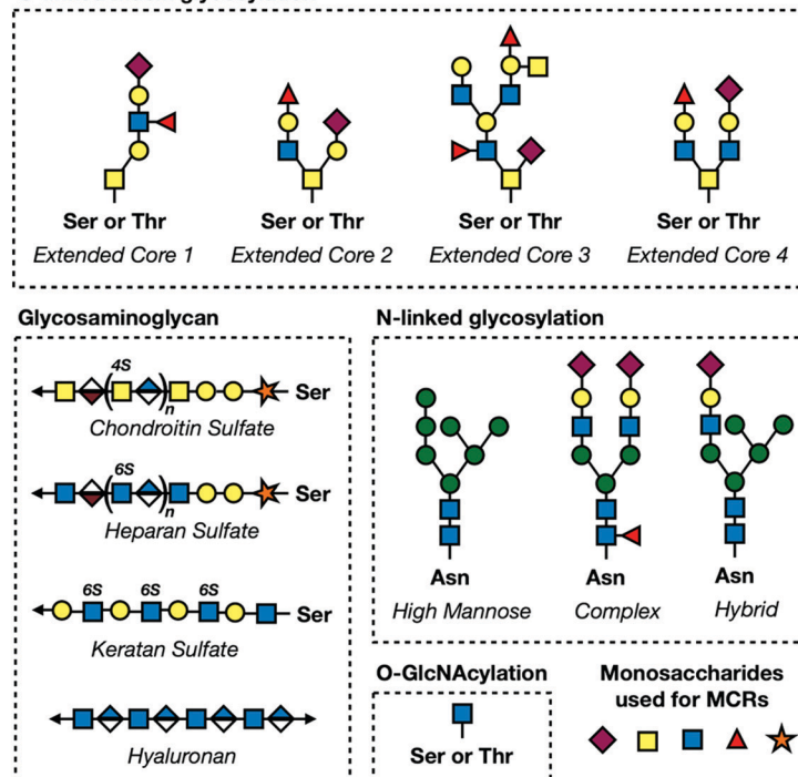
Fig. 1 (A) Common mammalian monosaccharide building blocks and their geometric codes. (B) Core structures for O-linked mucin, N-linked, GAG, and O-GlcNAcylation.
