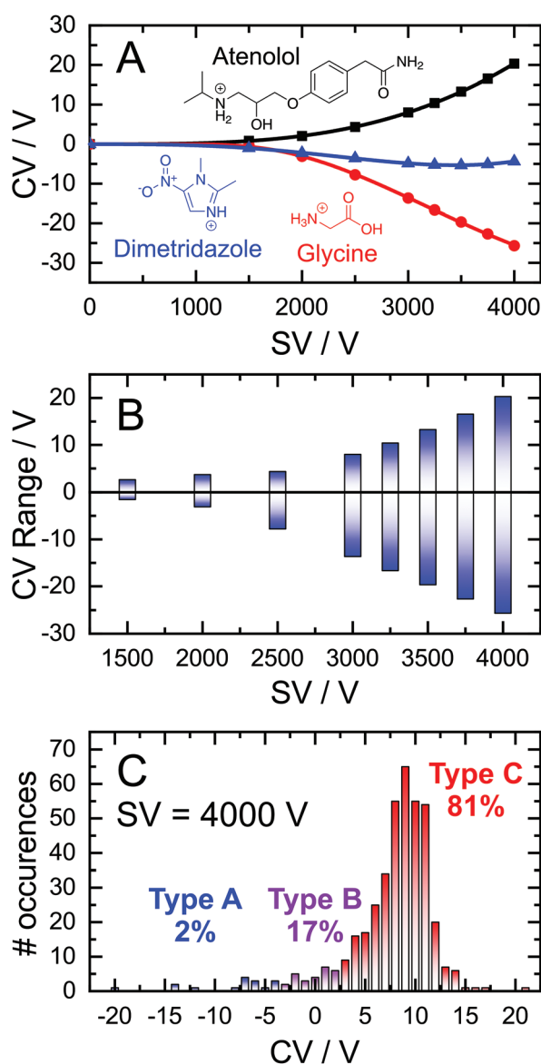
Fig. 1 (A) Dispersion curves for protonated atenolol (black squares), protonated dimetridazole (blue triangles), and protonated L-glycine (red circles). (B) The range of CV values for given SV values for the 409 molecules in our dataset and their distributions (C) at SV = 4000 V according to their Type A (blue), B (purple) or C (red).
