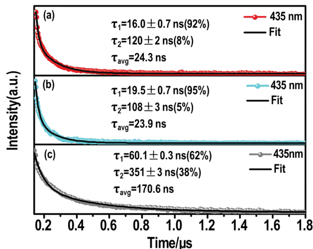
Fig. 4 Nanosecond time-resolve emission (ns-TE) decays and fittings of the (a) (S-\beta\text{-MPEA})_2\text{PbBr}_4 , (b) (R-\beta\text{-MPEA})_2\text{PbBr}_4 , and (c) ((rac)\text{-MPEA})_2\text{PbBr}_4 emission at 435 nm.
