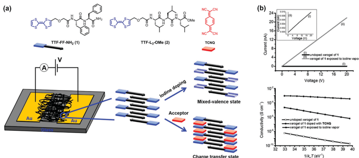
Fig. 1 (a) Schematic of conducting nanofibers composed of TTF-capped diphenylalanine and trileucine, doped with TCNQ as deposited across a gold electrode and their proposed self-assembly, (b) current–voltage (top) and conductivity (bottom) measurements showing significant enhancement upon exposure of TTF dried organogels to iodine vapour. 38 Copyright 2014, American Chemical Society.
