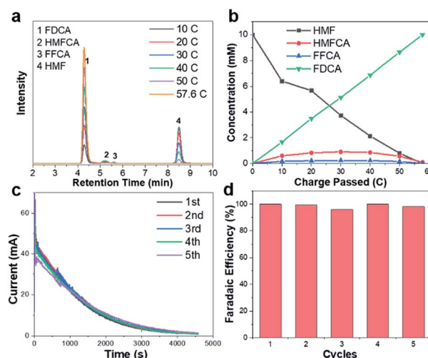
Fig. 3 (a) HPLC chromatogram traces of electrolyte during the electrochemical oxidation of HMF catalyzed by \text{Cu}_x\text{S}@ \text{Ni}_{0.75}\text{Co}_{0.25}\text{O}_m\text{H}_n at 1.32 V vs. RHE. (b) Concentration profiles of oxidation products with increasing charge. (c) Current-time curves and (d) faradaic efficiency towards FDCA in 5 successive runs.
