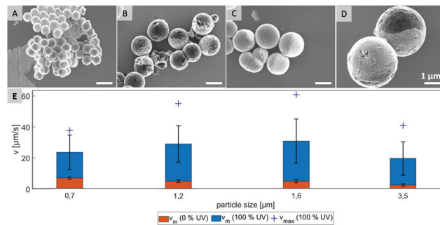
Fig. 3 SEM pictures of Janus particles with average sizes of 0.7 μm (A), 1.2 μm (B), 1.6 μm (C), 3.5 μm (D) and their velocities (E) in 0.5% H 2 O 2 solution ( v_m – mean velocity at given UV intensity, v_{max} – velocity of fastest particle), scale bar 1 μm.
