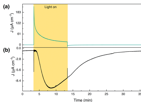
Fig. 4 Collector-generator experiment for a \text{TiCl}_4\text{-mTiO}_2|\text{DPP-Ru}/\text{CDCA} electrode prepared by immobilisation in MeOH solution (0.1 mM DPP-Ru and 20 mM CDCA). Conditions: NaOAc buffer (0.1 M, pH 5.6) with \text{NaClO}_4 (0.4 M), 100 \text{ mW cm}^{-2} , AM 1.5G, \lambda > 420 \text{ nm} , \text{N}_2 purged, room temperature. (a) Chronoamperometry photocurrent trace of the generator with an applied potential of +0.2 vs. NHE. (b) Chronoamperometry current trace of the collector with an applied potential of -0.6 vs. NHE.
