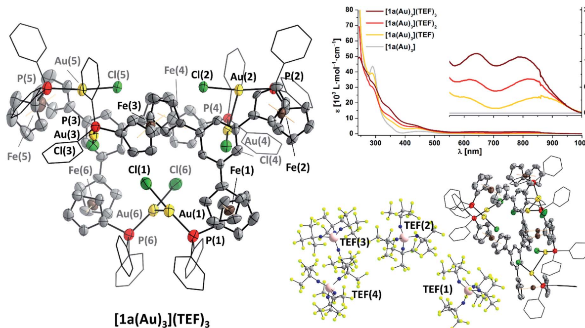
Fig. 6 (Left) Molecular structure of [1a(Au)_3]_2(TEF)_6 with partial atom numbering scheme. Thermal ellipsoids are set at the 50% probability level. For clarity, P -bound phenyl rings are depicted in wireframe style, and co-crystallised solvent, hydrogen atoms, and anions have been omitted. (Bottom right) Asymmetric unit of [1a(Au)_3]_2(TEF)_6 with the four localisable teflonate anions in ball-and-stick style. The presence of severely disordered teflonate anions TEF(5) and TEF(6) has been confirmed through their electron density and the unoccupied volume. (Top right) Stacked UV/Vis spectra of [1a(Au)_3](TEF)_n ( n = 0-3 ) in CH_2Cl_2 . The inset shows a magnification for the absorptions at long wavelength.
