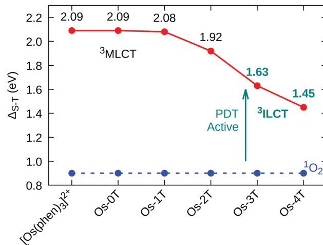
Fig. 6 Singlet-triplet energy gap ( \Delta_{S-T} ) for reference compound [\text{Os}(\text{phen})_3]^{2+} and Os-0T–Os-4T , in water, at the M06/6-31+G(d,p)/SDD level of theory.
