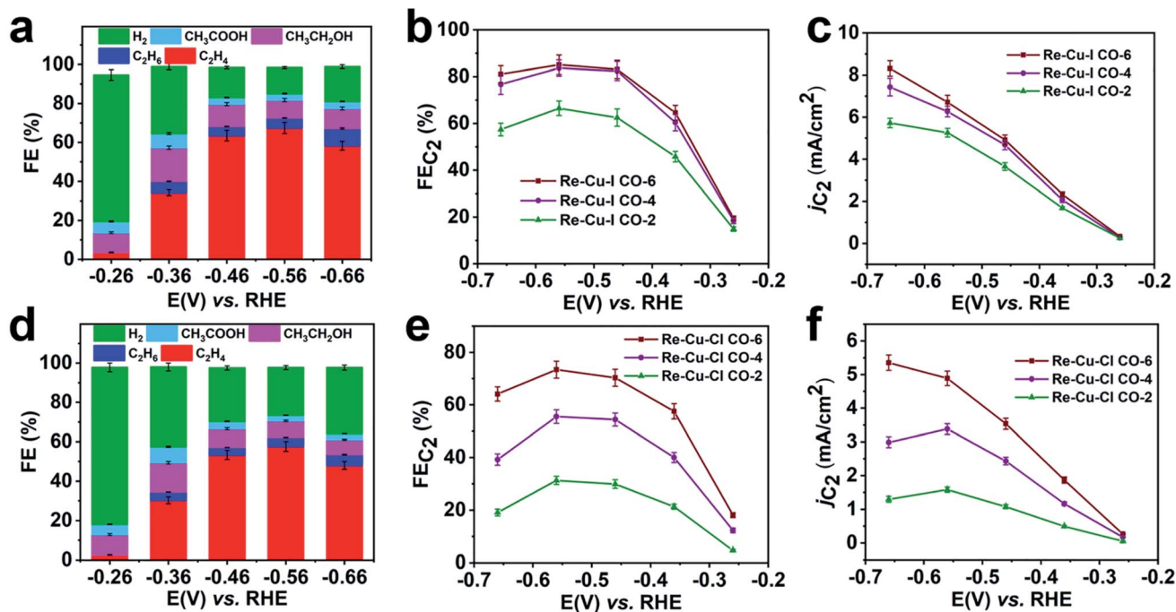
Fig. 4 Electrochemical CO reduction performance of Re-Cu-I, Re-Cu-Br and Re-Cu-Cl. FE of carbon products from CO electroreduction on Re-Cu-I (a) and Re-Cu-Cl (d) with a CO flow rate of 6 mL min -1 at potentials ranging from -0.26 V to -0.66 V vs. RHE. FE of C 2 products from CO electroreduction on Re-Cu-I (b) and Re-Cu-Cl (e) with CO flow rates of 6 mL min -1 , 4 mL min -1 , and 2 mL min -1 at potentials ranging from -0.26 V to -0.66 V vs. RHE. (c) Partial current density of C 2 products from CO electroreduction on Re-Cu-I (c) and Re-Cu-Cl (f) with CO flow rates of 6 mL min -1 , 4 mL min -1 , and 2 mL min -1 at potentials ranging from -0.26 V to -0.66 V vs. RHE.
